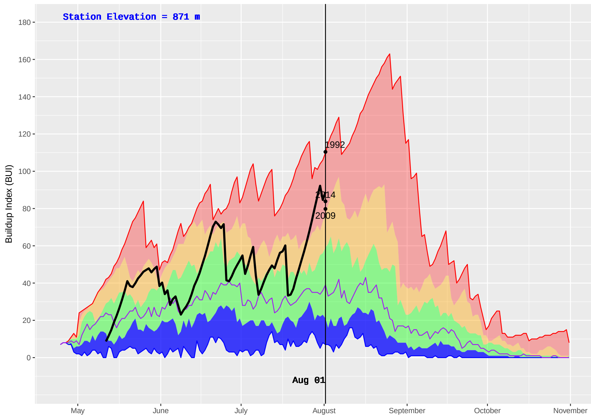
SUSTUT (156) : Historical (1989–2016) and Current (2018) Daily Buildup Index (BUI)
